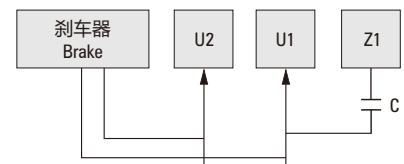
100W/200W顺时针接法/CW Connection
